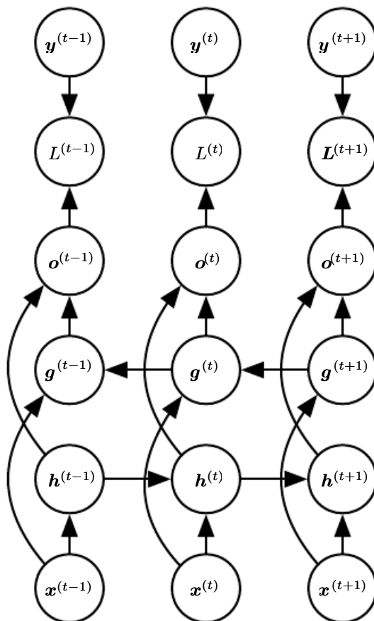
Figure 10.11: Computation of a typical bidirectional recurrent neural network, meant to map input sequences \mathbf{x} to target sequences \mathbf{y} , with loss L^{(t)} at each step t . The \mathbf{h} recurrence propagates information forward in time (towards the right) while the \mathbf{g} recurrence propagates information backward in time (towards the left). Thus at each point t , the output units \mathbf{o}^{(t)} can benefit from a relevant summary of the past in its \mathbf{h}^{(t)} input and from a relevant summary of the future in its \mathbf{g}^{(t)} input.
