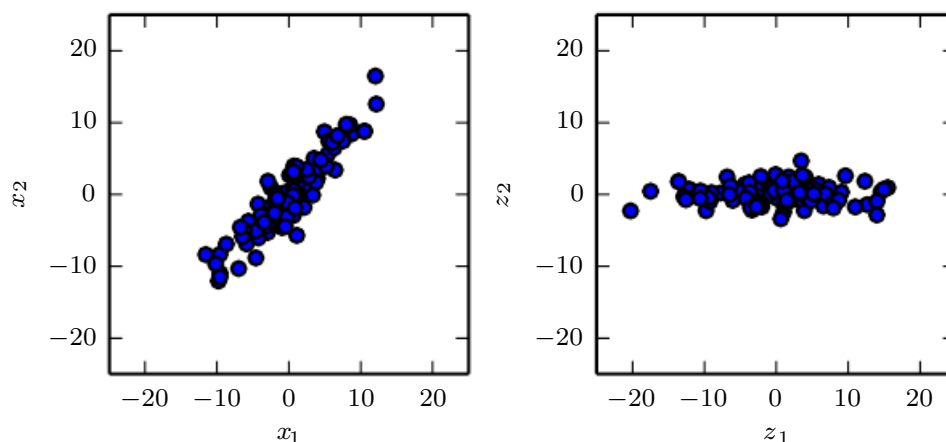
Figure 5.8: PCA learns a linear projection that aligns the direction of greatest variance with the axes of the new space. ( Left )The original data consists of samples of \mathbf{x} . In this space, the variance might occur along directions that are not axis-aligned. ( Right )The transformed data \mathbf{z} = \mathbf{x}^\top \mathbf{W} now varies most along the axis z_1 . The direction of second most variance is now along z_2 .
