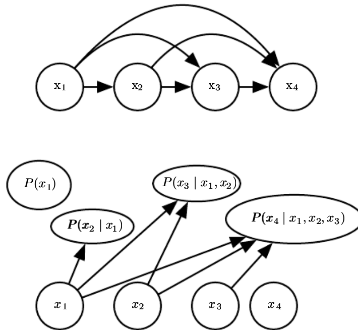
Figure 20.8: A fully visible belief network predicts the i -th variable from the i - 1 previous ones. ( Top )The directed graphical model for an FVBN. ( Bottom )Corresponding computational graph, in the case of the logistic FVBN, where each prediction is made by a linear predictor.
